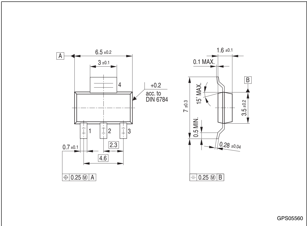
Figure 4 PG-SOT223-4-11 (Plastic Small Outline Transistor)
